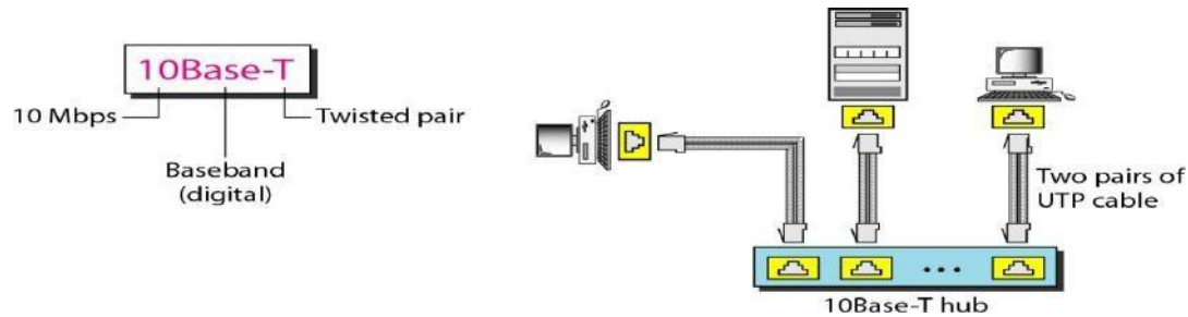
10Base-T implementation
